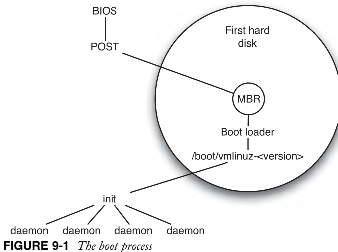
FIGURE 9-1 The boot process
