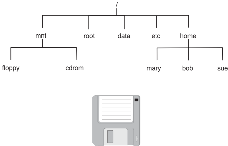
FIGURE 6-1 The directory structure prior to mounting
